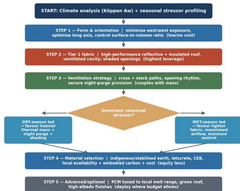
Figure 5. A staged decision framework for prioritising passive parameters in savanna residential design
