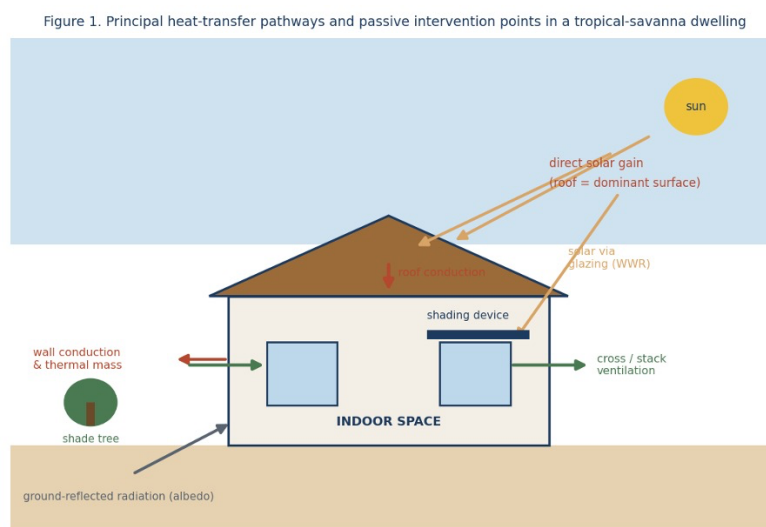
Figure 1. Principal heat-transfer pathways and the corresponding passive intervention points in a tropical-savannah dwelling. The roof is the dominant solar-gain surface, while cross and stack ventilation provide the principal heat-removal mechanism.
