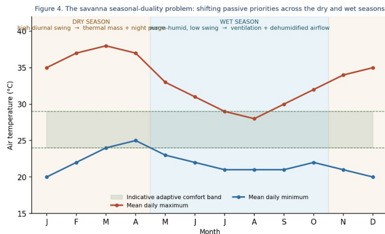
Figure 4. The savannah seasonal-duality problem. The collapse of the diurnal range between the dry and wet seasons inverts the relative value of thermal mass and ventilation, motivating adaptive rather than fixed envelopes.
