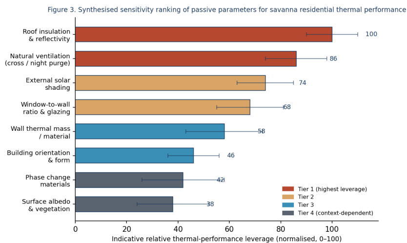
Figure 3. Synthesised sensitivity ranking of passive parameters. Bars show indicative relative leverage and whiskers the spread of reported effects across the corpus; the ranking weights savannah and Nigerian residential evidence most heavily.
